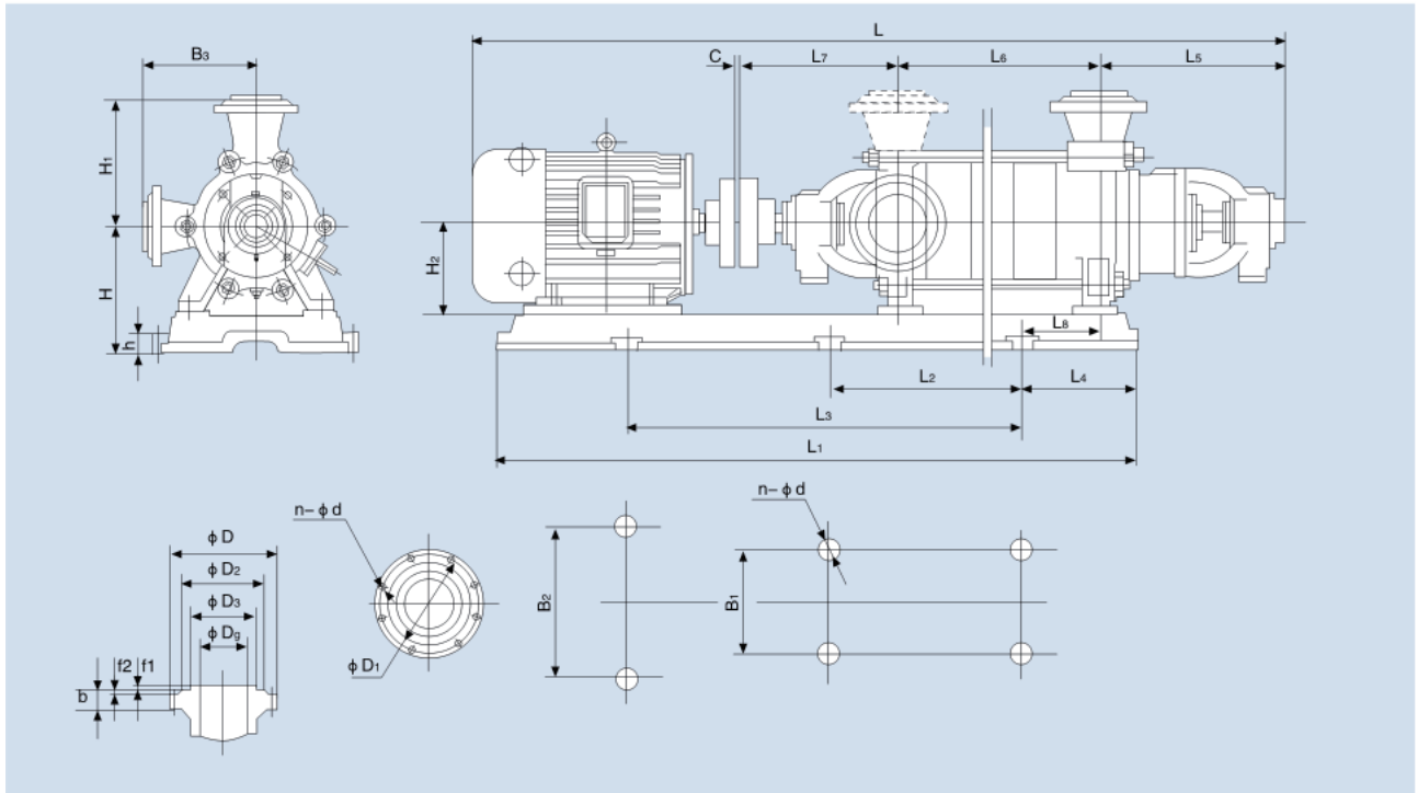
CMB 型泵外形安装图(本身底座) (With Pump Base)
