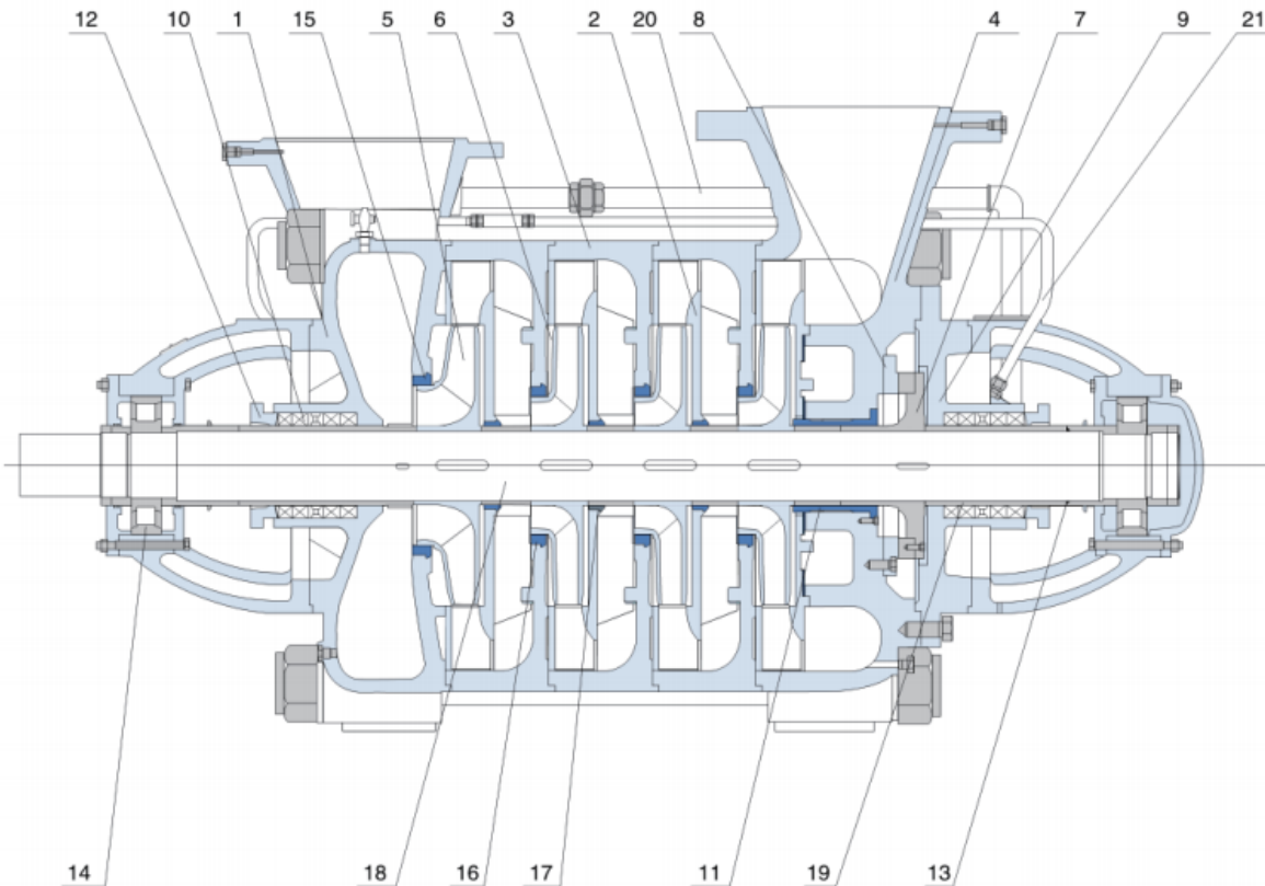
Structural Arrangement
