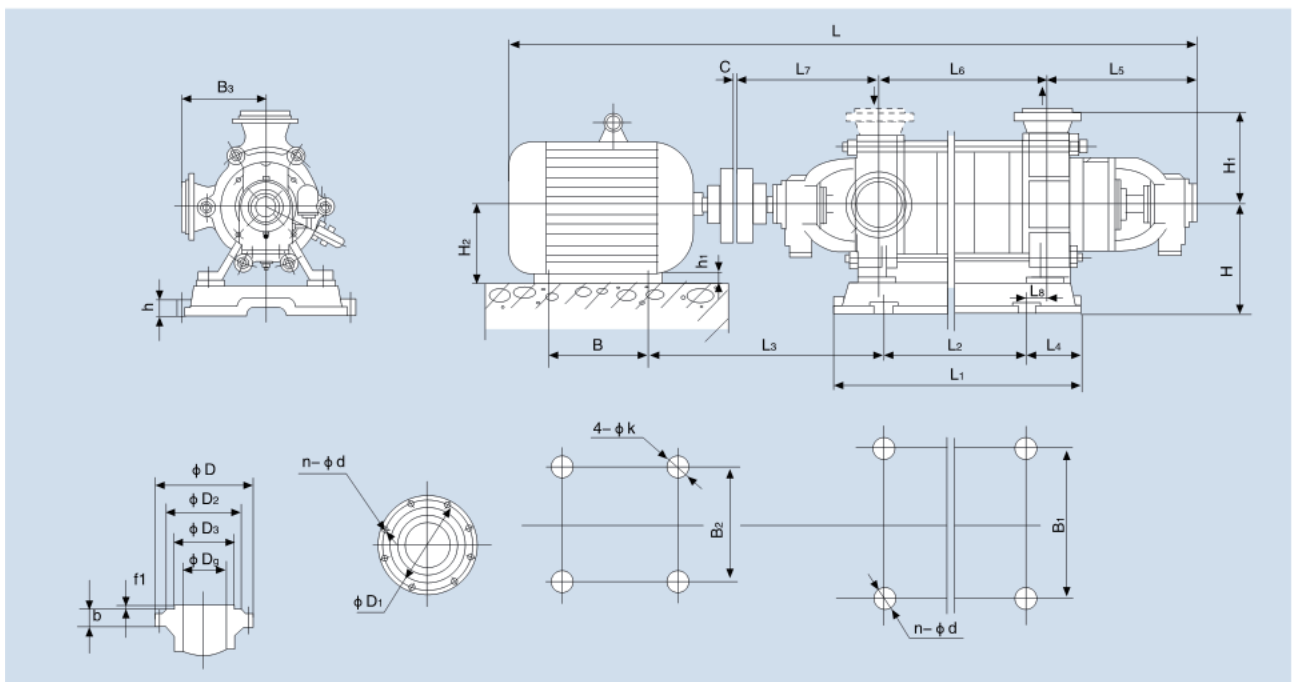
CMB 型泵外形安装图(本身底座) (With Pump Base)
